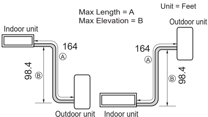
Figure 49: Typical LH188HV1, LH248HV1 System Layout.
