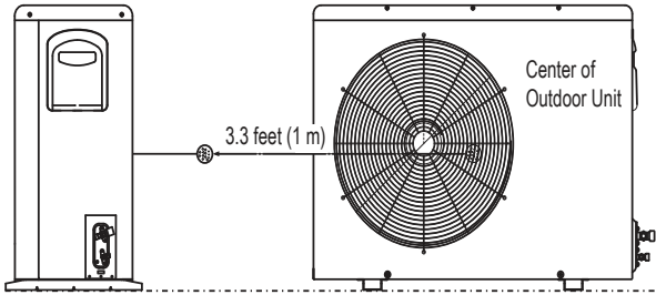
Figure 7: Mid Static Ducted Outdoor Unit Sound Pressure Level Measurement Location.
