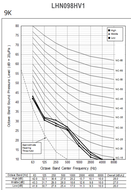
Figure 9: Ducted Indoor Unit Sound Pressure Level Diagrams.
