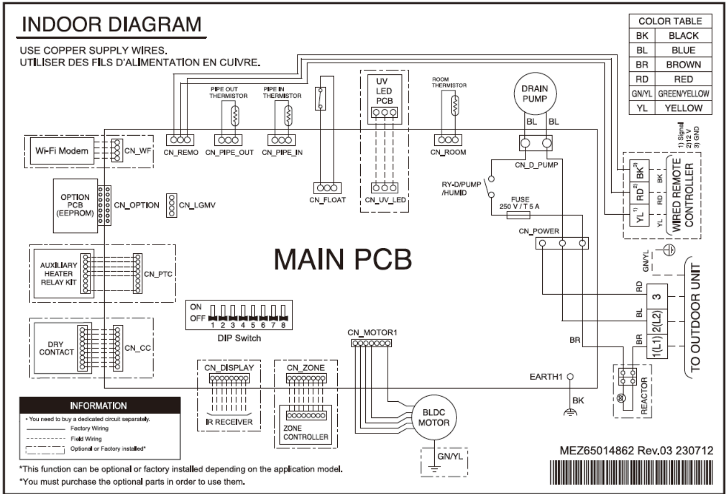
Figure 16: LHN098HV1, LHN128HV1, LHN188HV1, LHN248HV1 Mid Static Ducted Indoor Unit Wiring Diagram.
