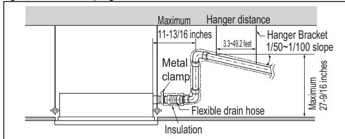
Figure 35: Drain Piping Installation Dimensions.
