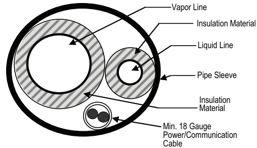
Figure 37: Typical Arrangement of Refrigerant Pipe and Cable(s) in a Utility Conduit.
