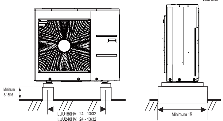
Figure 44: Bolting the LUU180HV, LUU240HV Outdoor Units to the Platform (Appearance May Vary).
