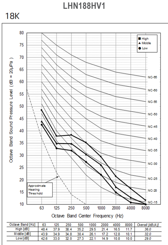
Figure 10: Ducted Indoor Unit Sound Pressure Level Diagrams.
