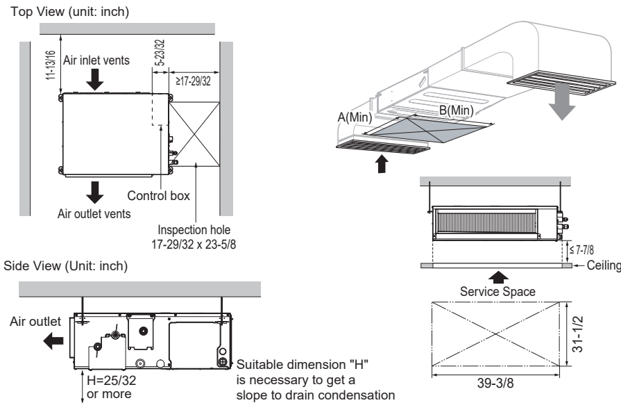
Figure 33: Mid Static Ducted IDU Access Panel Required Dimensions.
