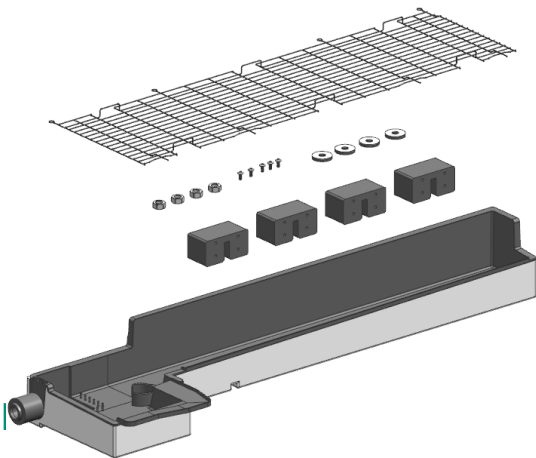
Figure 27: Drain Pan Heater.
