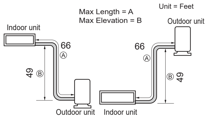
Figure 48: Typical LH098HV1, LH128HV1 System Layout.
