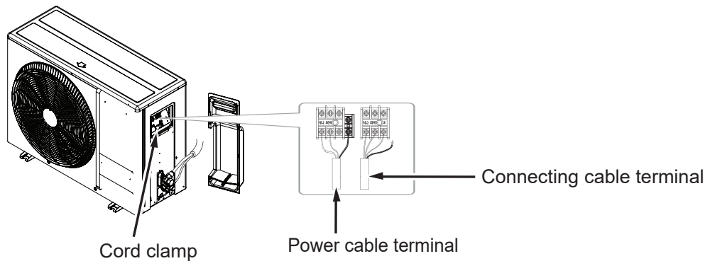
Figure 18: LUU090HV, LUU120HV ODU Terminal Block Location.
