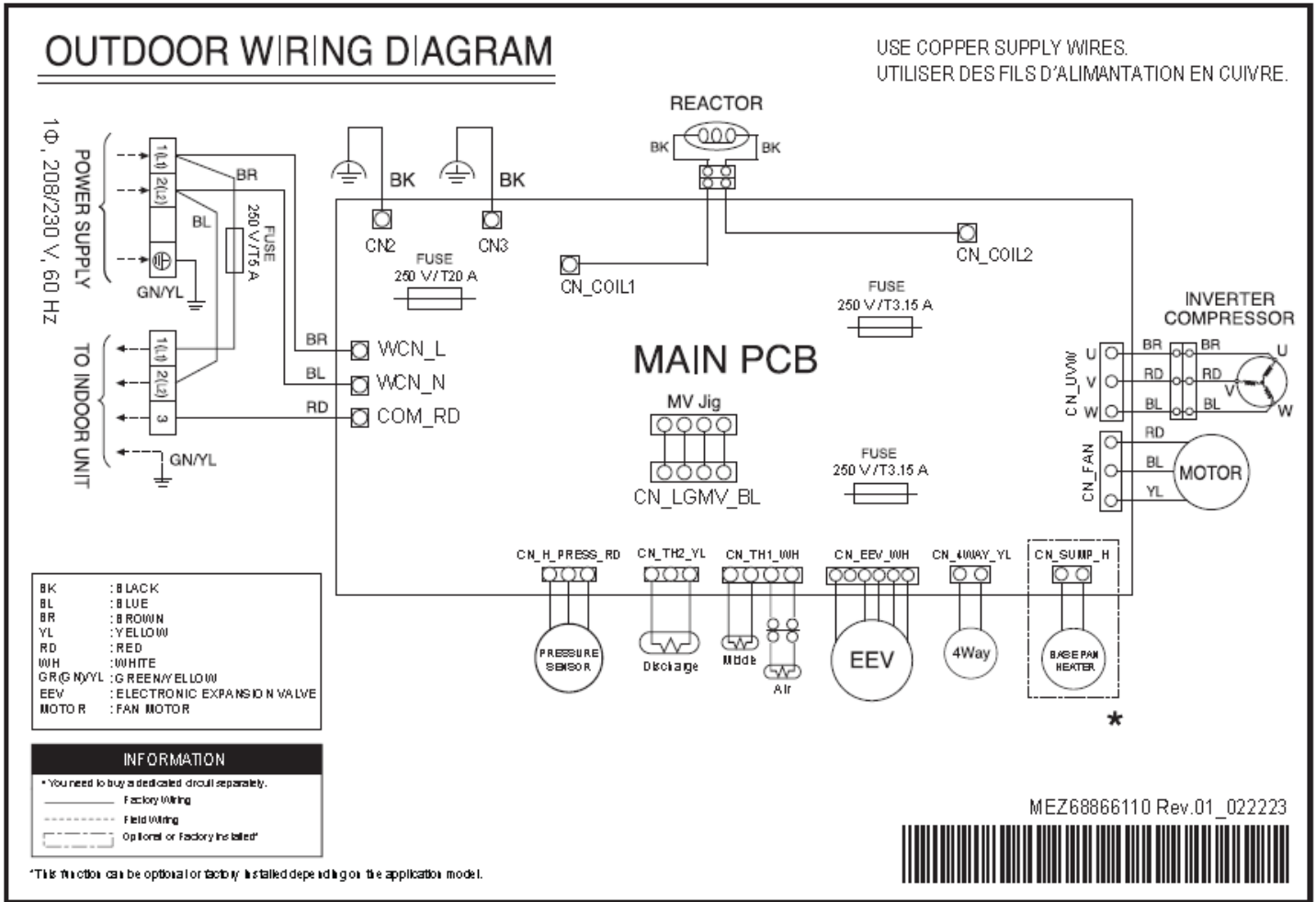
Figure 14: LUU090HV, LUU120HV Outdoor Unit Wiring Diagram.
