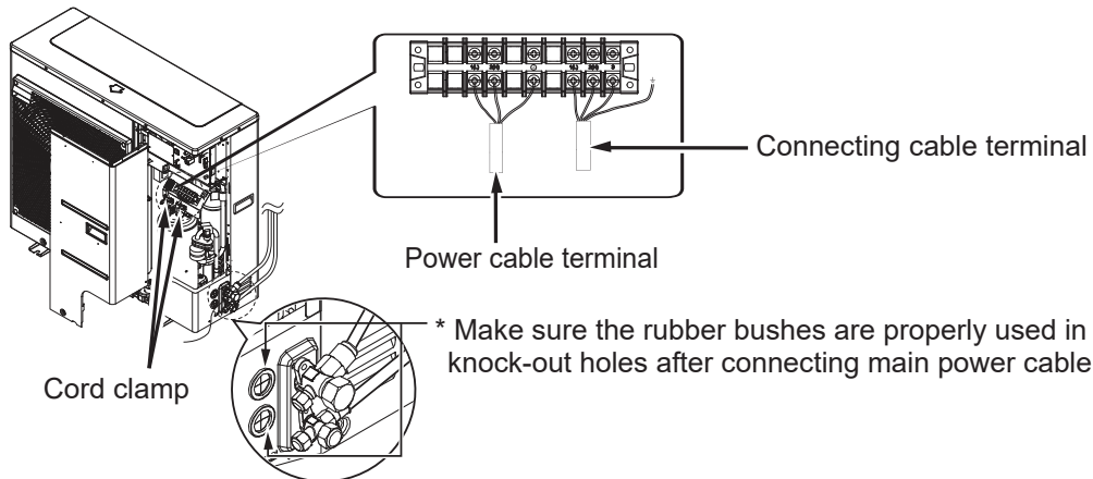
Figure 19: LUU180HV, LUU240HV ODU Terminal Block Location.
