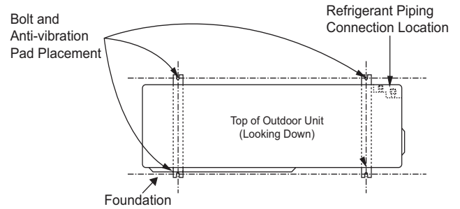
Figure 46: Close up of Bolt Attachment.
