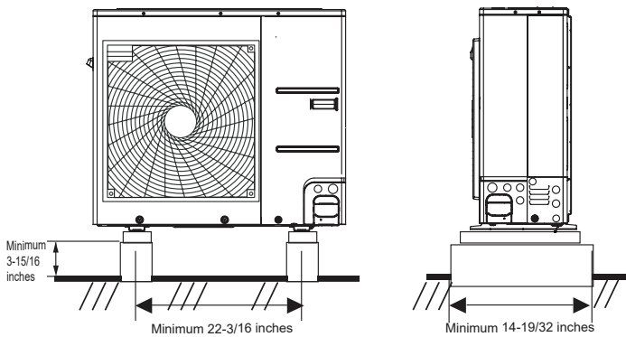
Figure 43: Bolting the LUU090HV, LUU120HV Outdoor Units to the Platform (Appearance May Vary).
