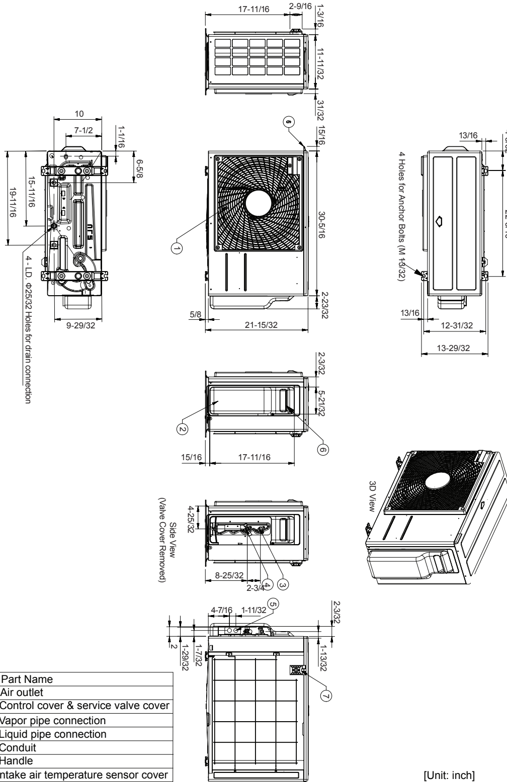
Figure 4: LUU090HV, LUU120HV Dimensions.
