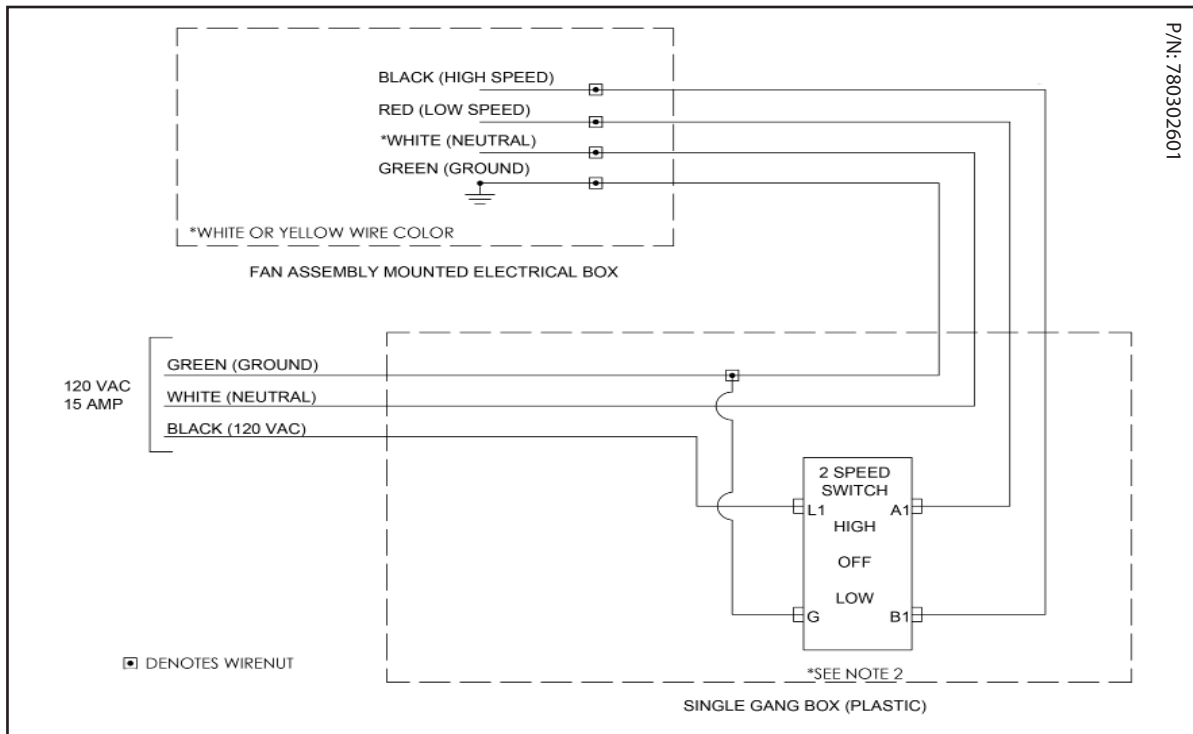
DIAGRAM 2: For CA2-CA5 Models with 2 Speed Wall Control
