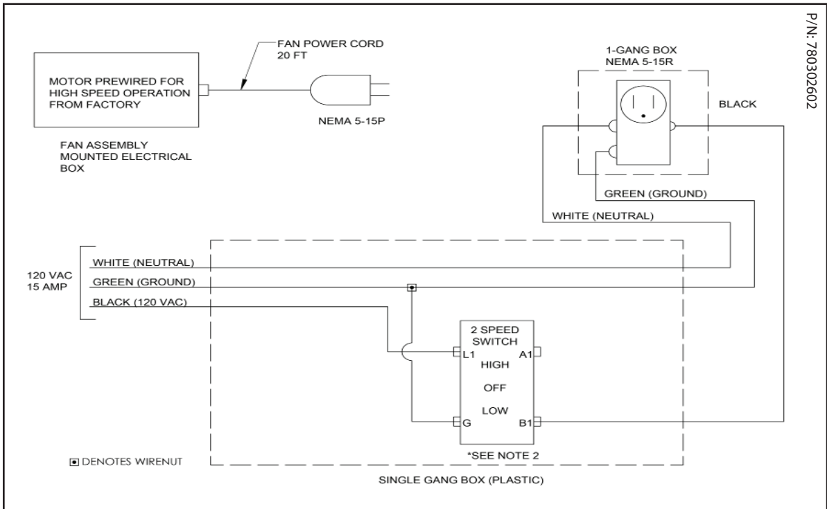
DIAGRAM 1: For CA2-CA5 Models with Single Speed & hardwired to Fan Assembly
