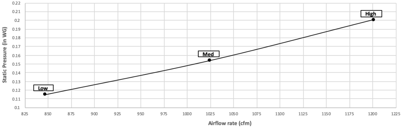
PEAD-A36AA8 with Filter Box FBM2-4-A
