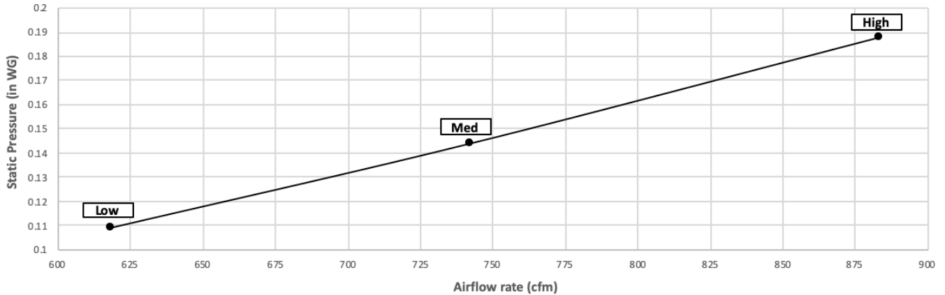
PEFY-P24, P27, P30NMAU-E4 with Filter Box FBM2-3-A
