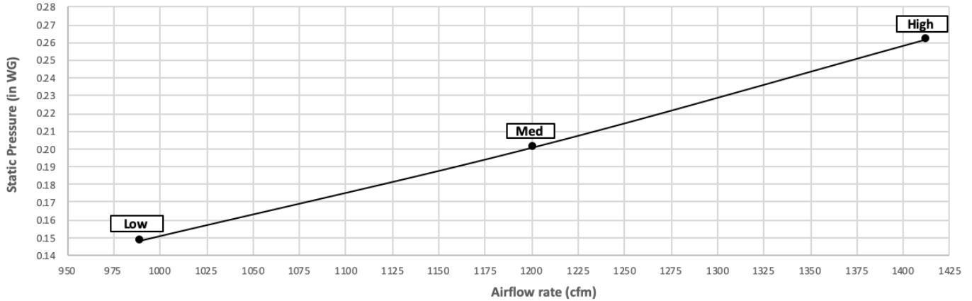
PEFY-P48NMAU-E4 with Filter Box FBM2-4-A
