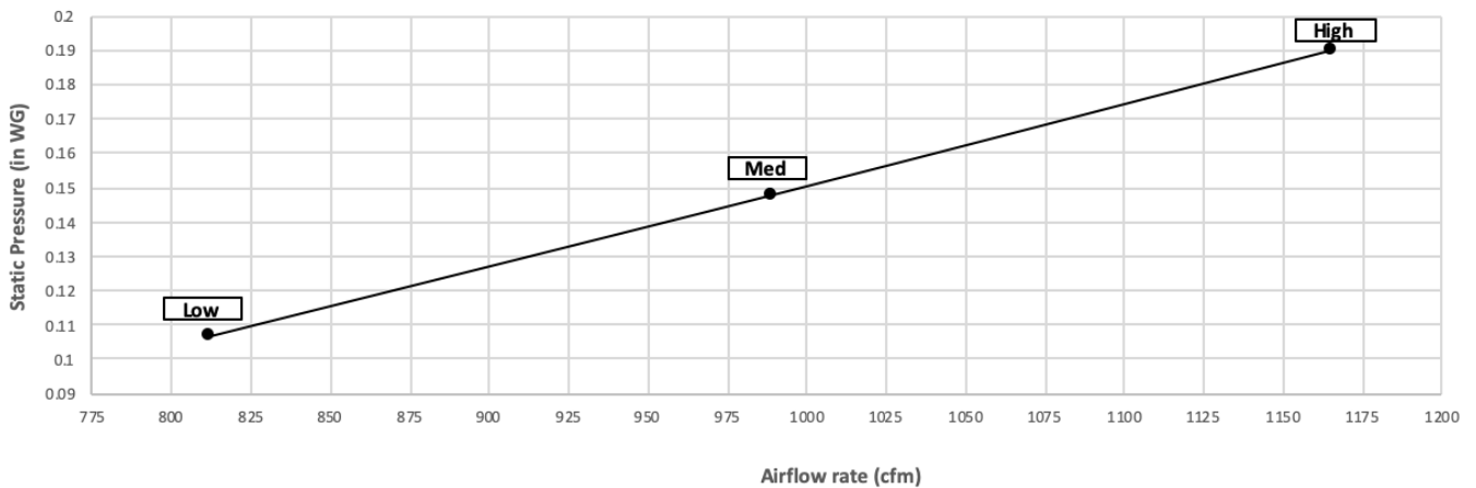
PEFY-P36NMAU-E4 with Filter Box FBM2-4-A
