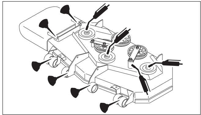
Figure 21. Deck Lubrication
