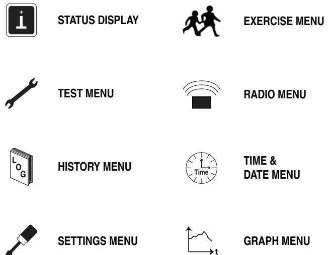
Figure 16 — Menu System
