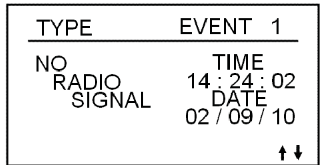
Figure 18 — History Menu
