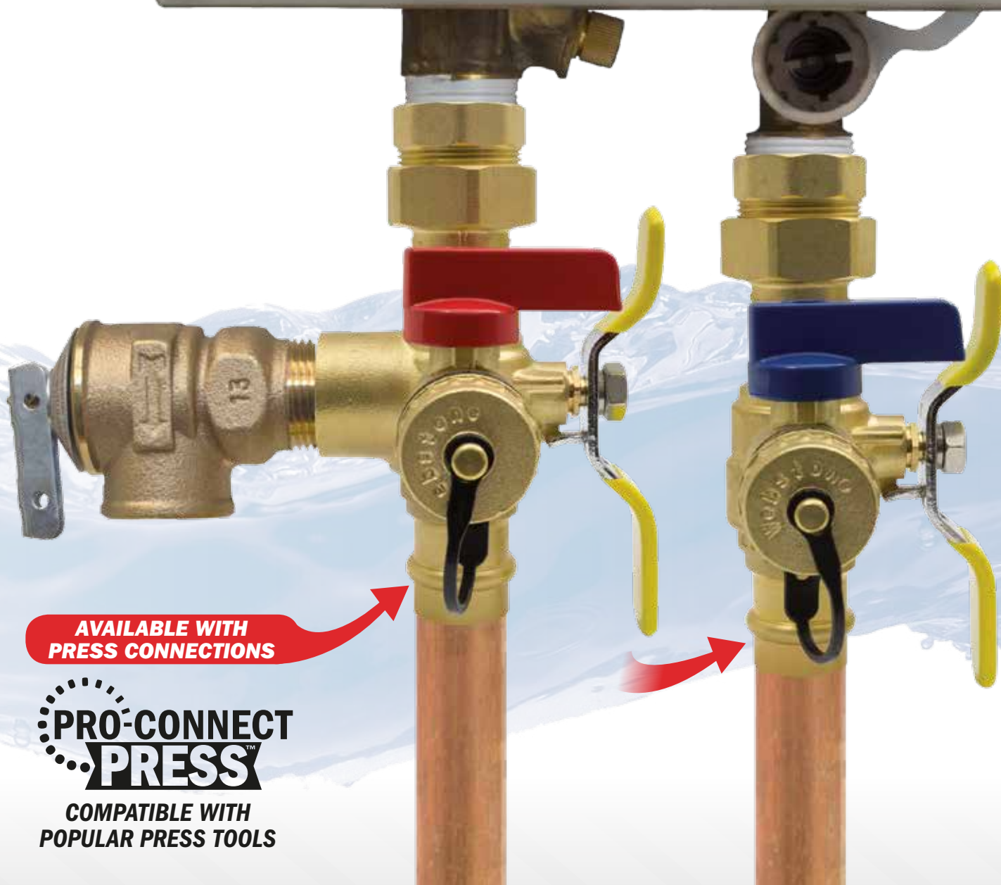
RESIDENTIAL PRESSURE RELIEF VALVE
