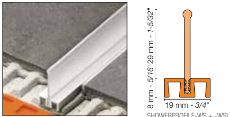
SHOWERPROFILE-WS + -WSL
