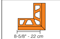
Outside corner, 135°
