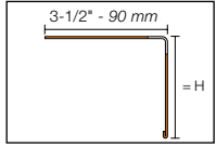
Outside corner
