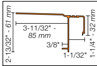
Outside corner, 90°
