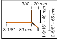
Outside corner, 90°
