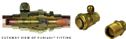
CUTAWAY VIEW OF FitRight™ FITTING
