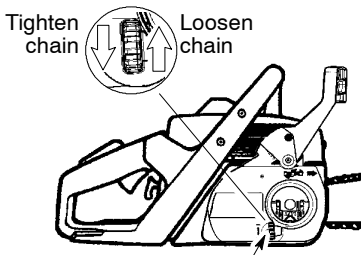
Adjusting Wheel
