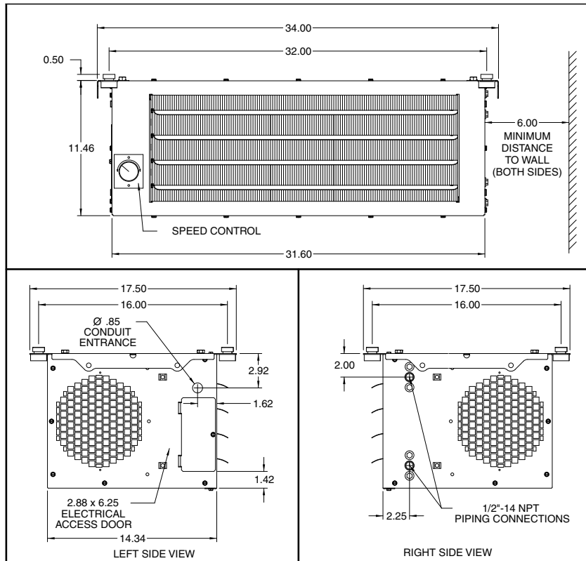
Figure 4.1 - Model HDD Dimensions (inches)
