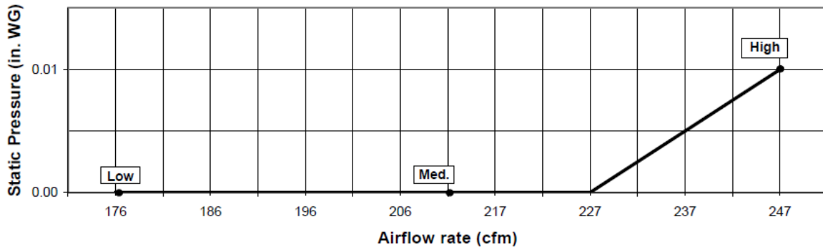
SEZ-KD09NA4 with Filter Box FBL1-1
