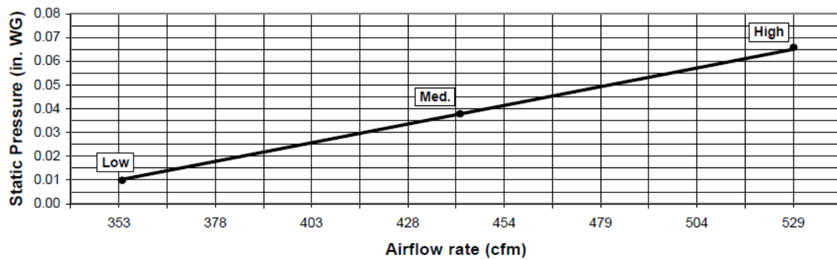
SEZ-KD15NA4 with Filter Box FBL1-2
