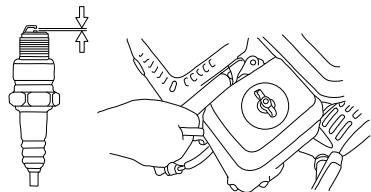
Figure 4-10. Spark Plug
