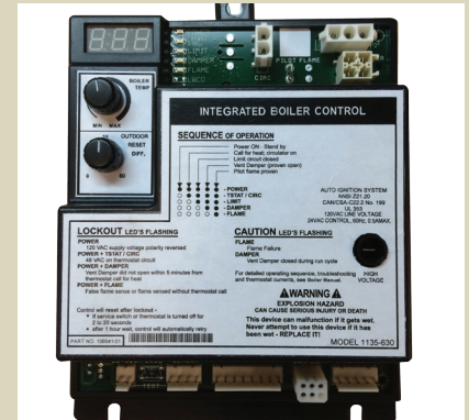
Integrated Boiler Control with diagnostics
