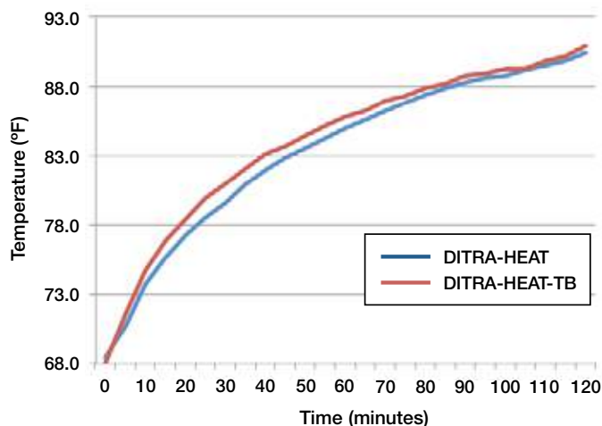
Figure 2 - DITRA-HEAT-TB Performance over Wood
