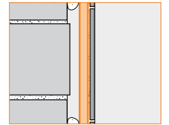
12.1 Schluter®-KERDI-BOARD
